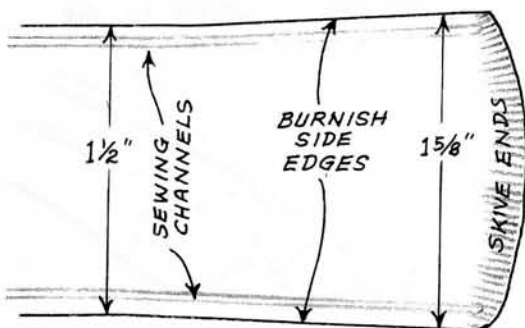
COVER LEATHER
