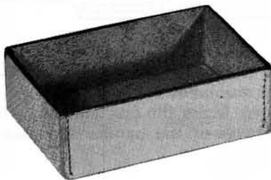
Completed box, using the measurements on the opposite page. Miter joint corners.
