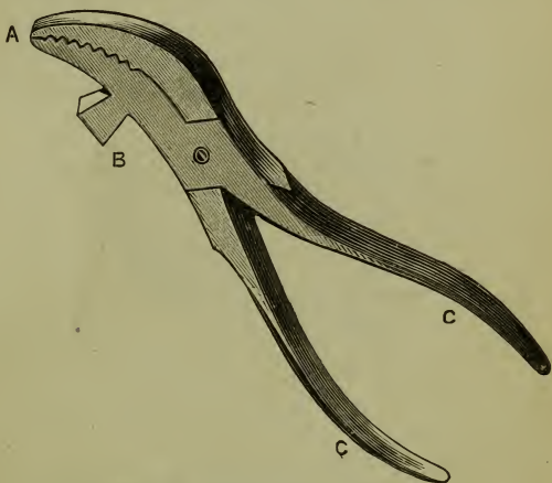
Fig. 88.—Shoemaker's Pincers.
