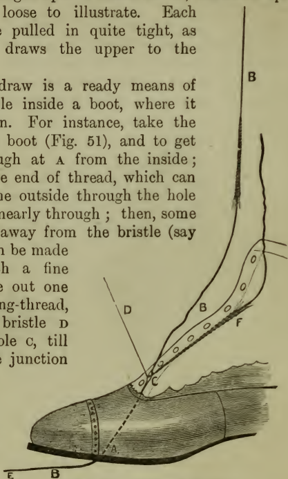
Fig. 51.—Stitch Drawing.
