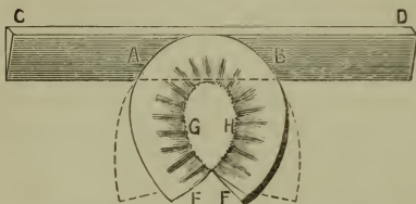
Fig. 104.—Turning the Split-lift.
