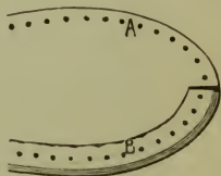
Fig. 120.—Pegged Seat and Split-lift.
