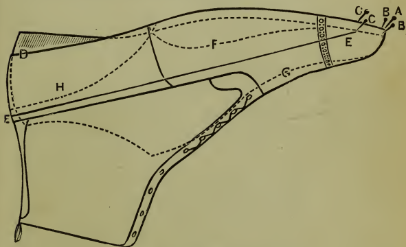
Fig. 84.—Ready for Lasting.
