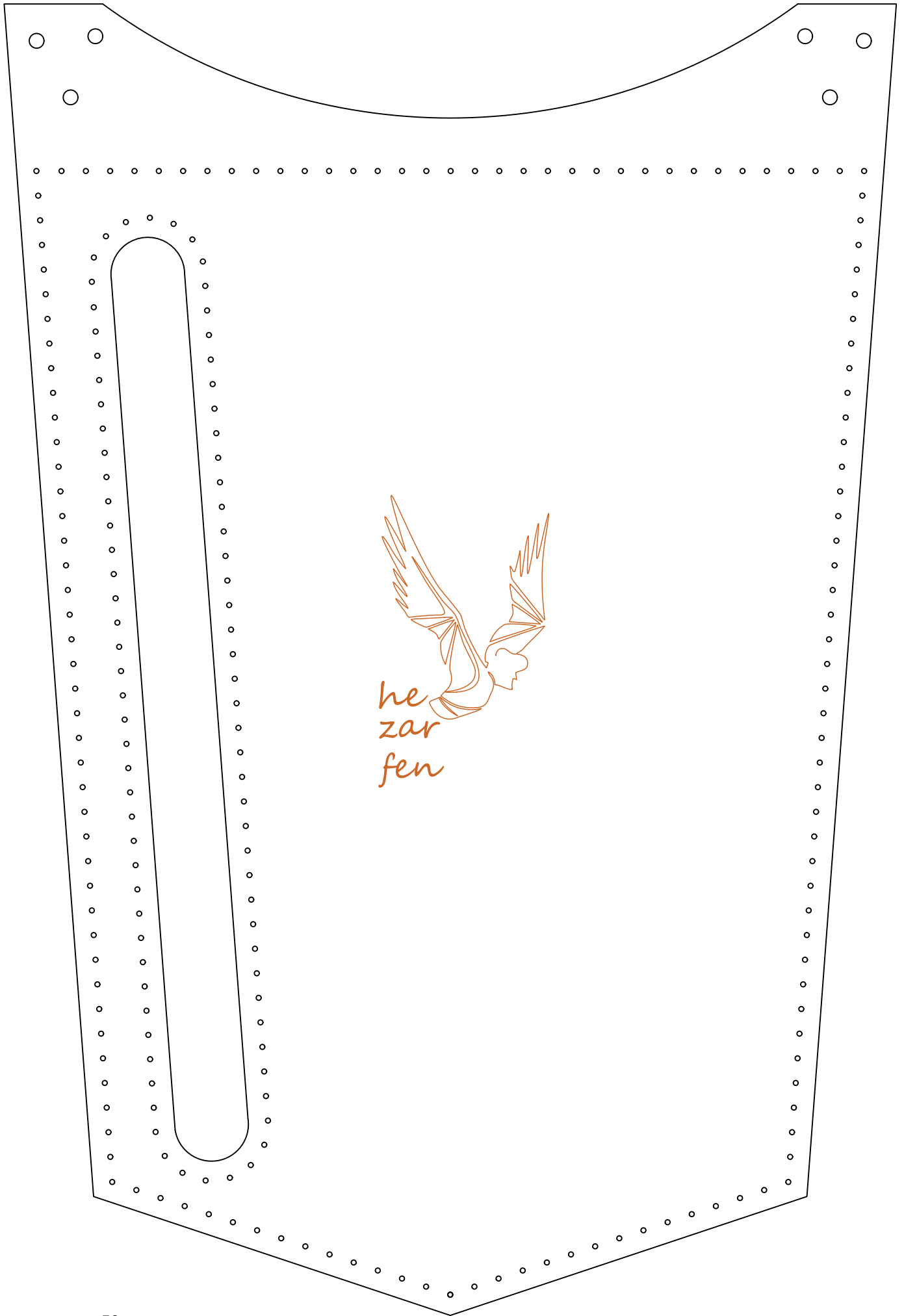
hezarfen art hitman bag pattern Size : 177 * 237 mm - 7" * 9.3"
