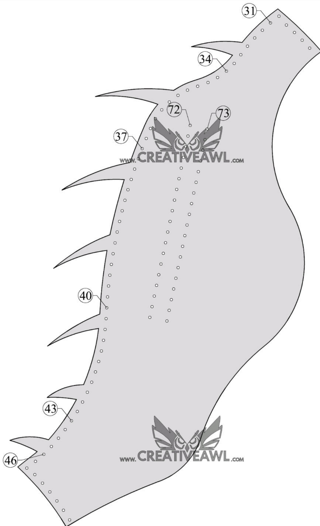
Leather Dragon - torso component -
