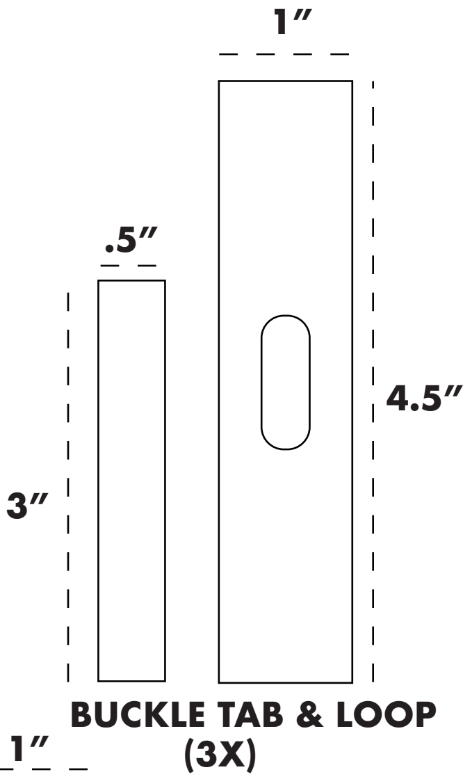
SHIELD AND TAB (2X)
