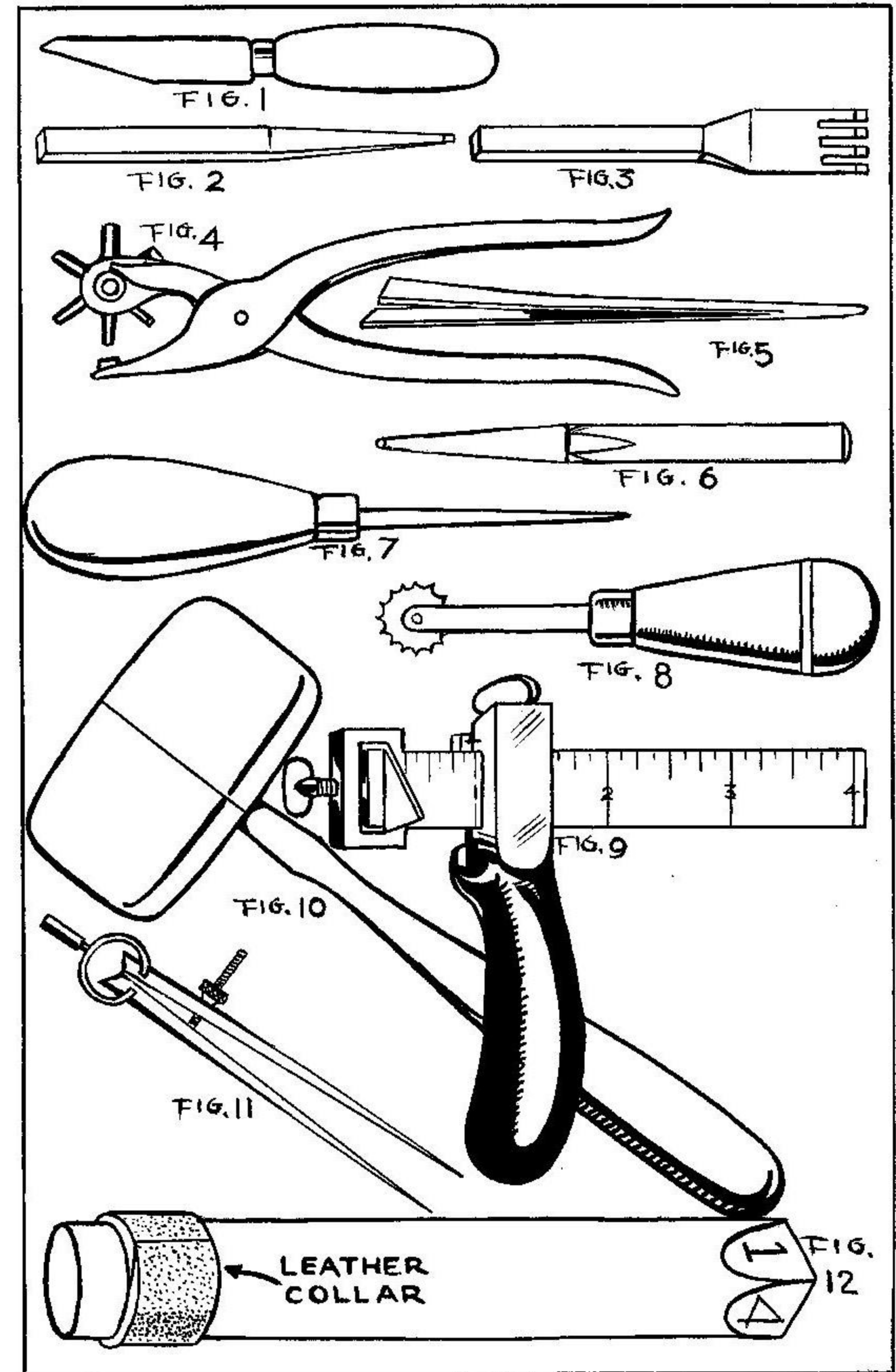
PLATE 1—Leather Braiding Tools.
