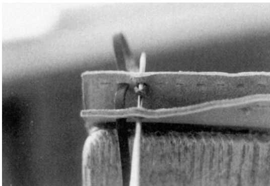
Fig 98 Second stitch, needle passing through slit in thong tab end. (For clarity, the first loop has not been pulled tight here.)
