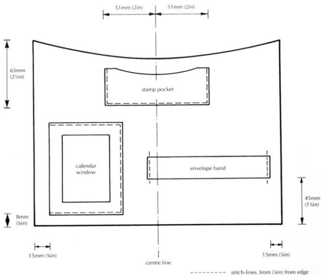
Fig 147 Plan and dimensions of left-hand assembly (LHA).
