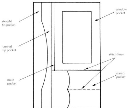
Fig 139 Bight pocket assembly (RPA).
