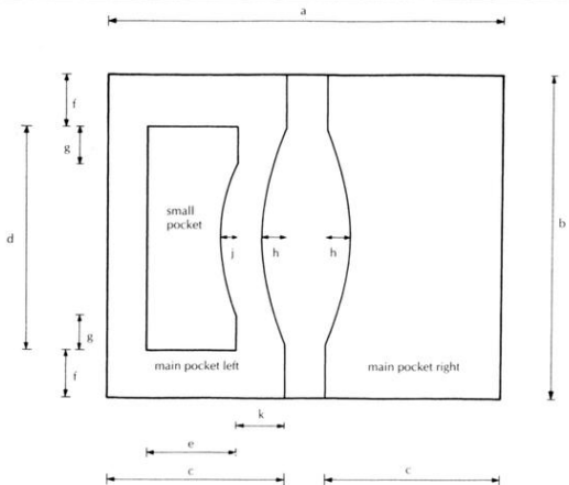
Fig 30 Constructional diagram for making a wallet.
