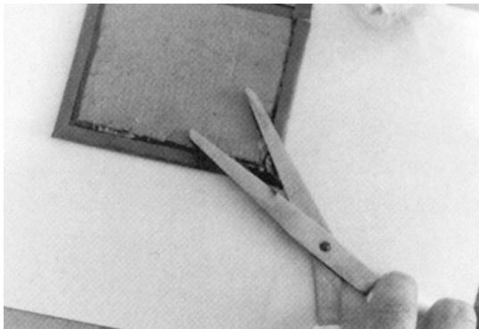
Fig 26 Trimming off excess material at the corner using scissors - for thin leathers or rexine only.
