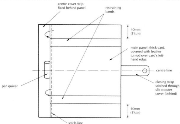
Fig 146 Plan of right-hand assembly (RHA).
